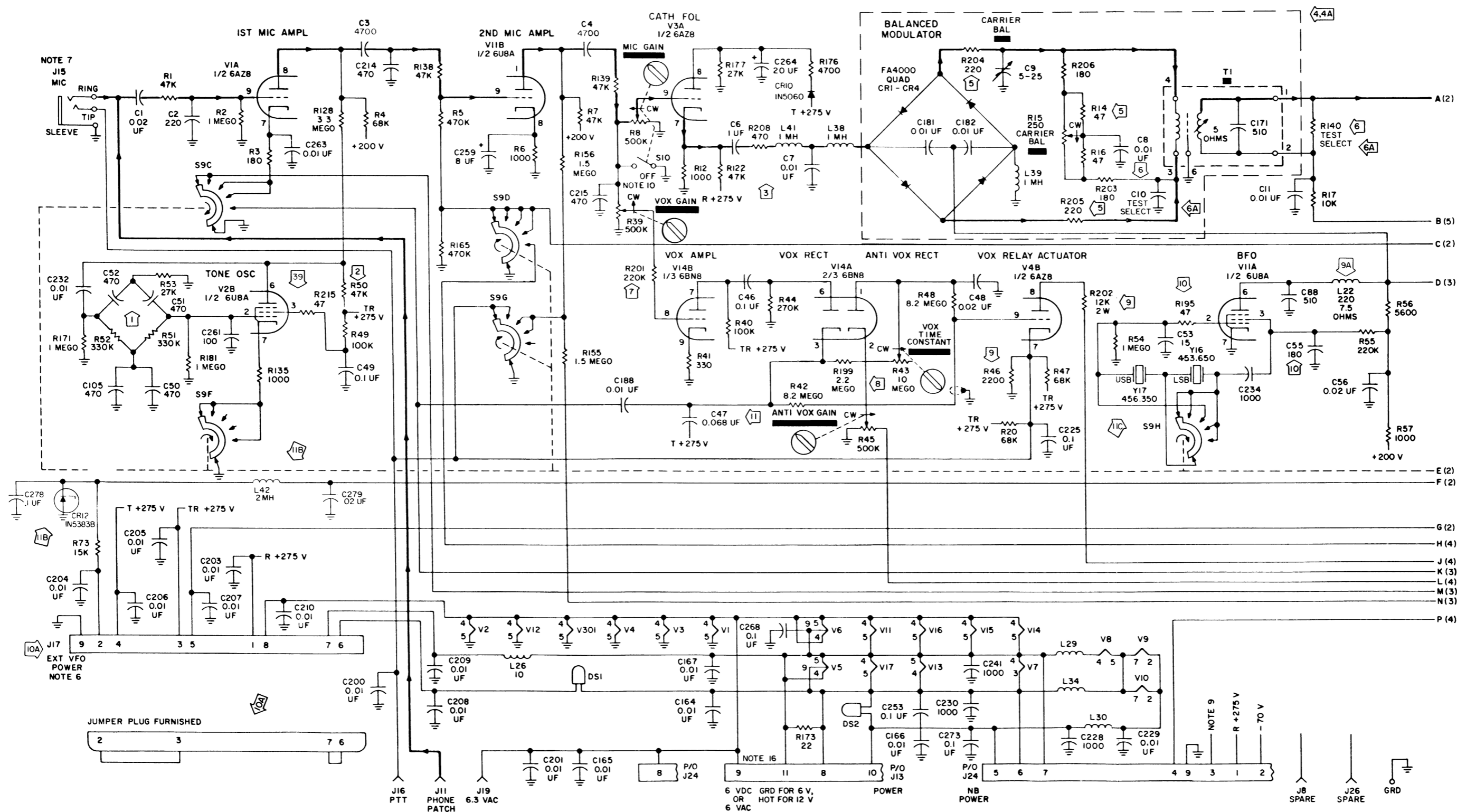
KWM-2 and KWM-2A Transceivers, Schematic Diagram Figure 7-1 (Sheet 1 of 5)
